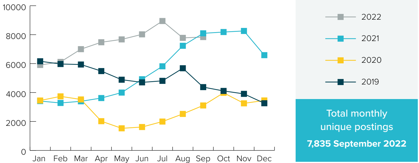
Job postings - Managers and Directors in Retail and Wholesale
